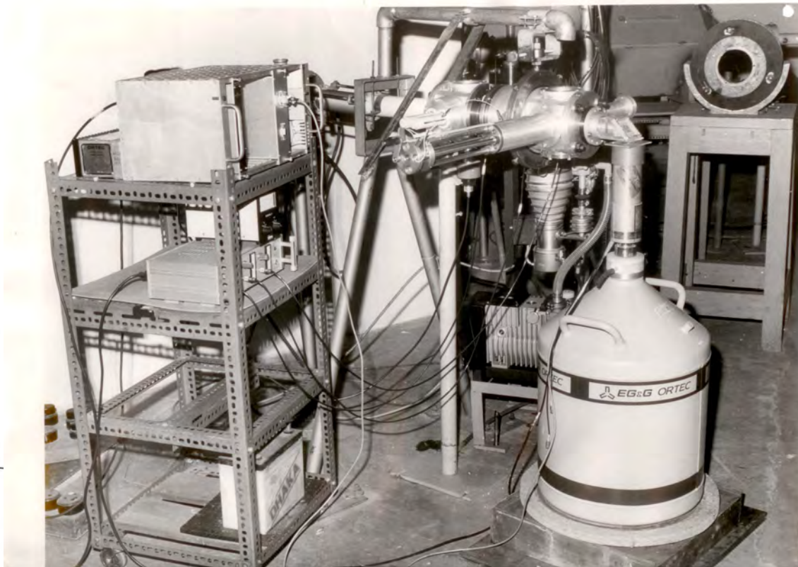
PHOTO OF THE MAIN EXPERIMENTAL SETUP
